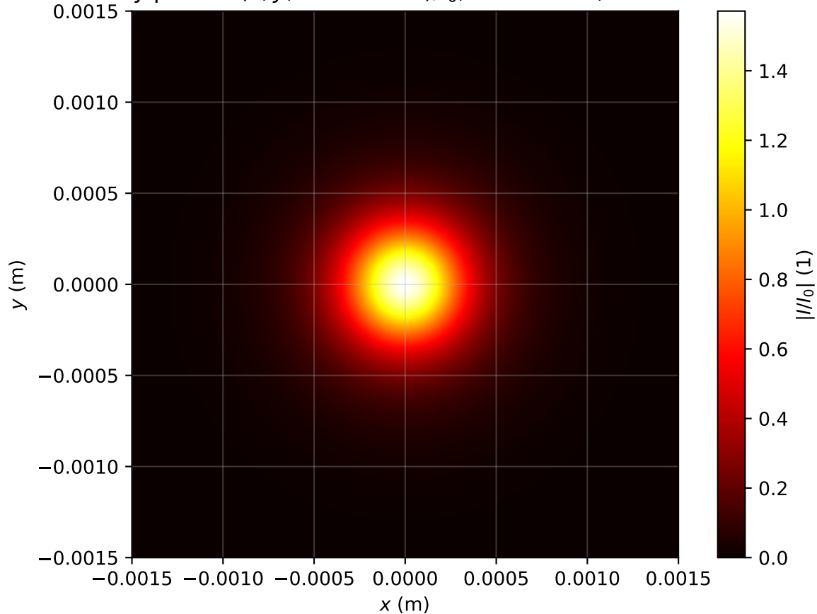
Intensity profile I(x, y, z = 1.513m)/I_0 , Pin=0.9Pcr, artificial time
